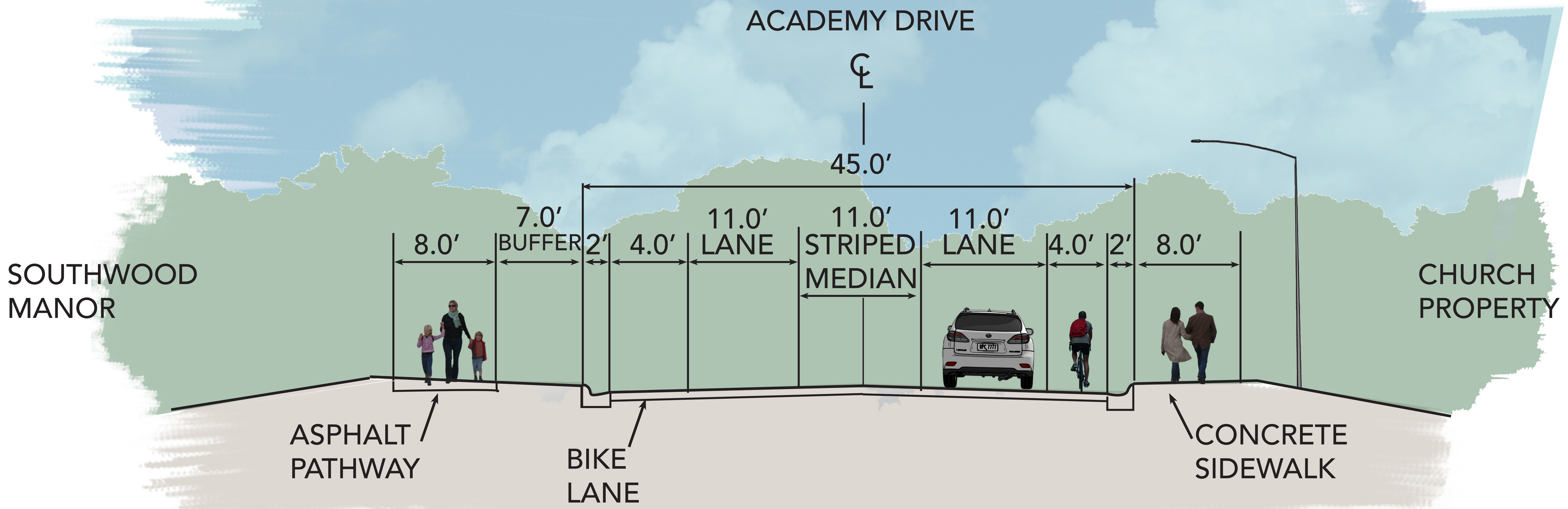
PROPOSED ACADEMY DRIVE ROADWAY SECTION
